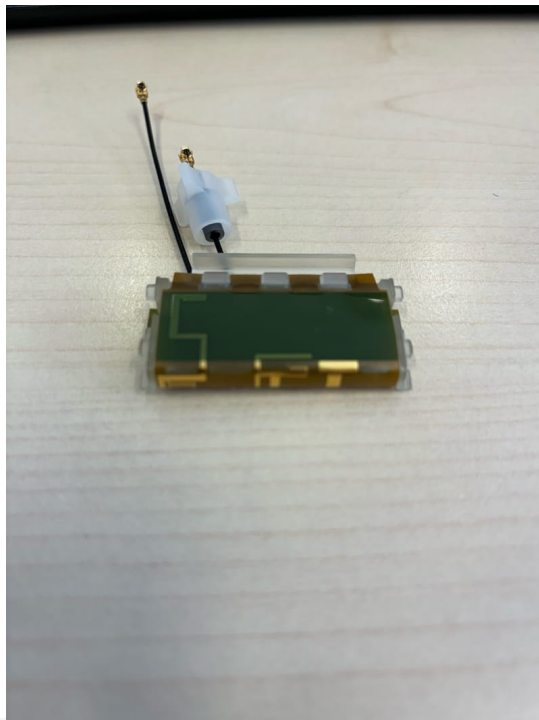
Photo 11: 453564521801 antenna
