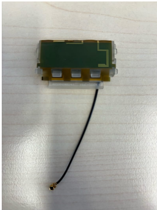
Photo 13: 453564682551 antenna
