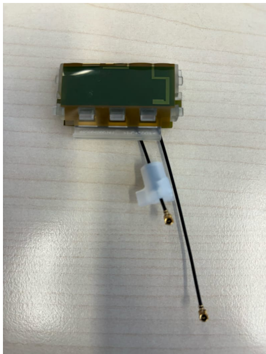
Photo 12: 453564521801 antenna
