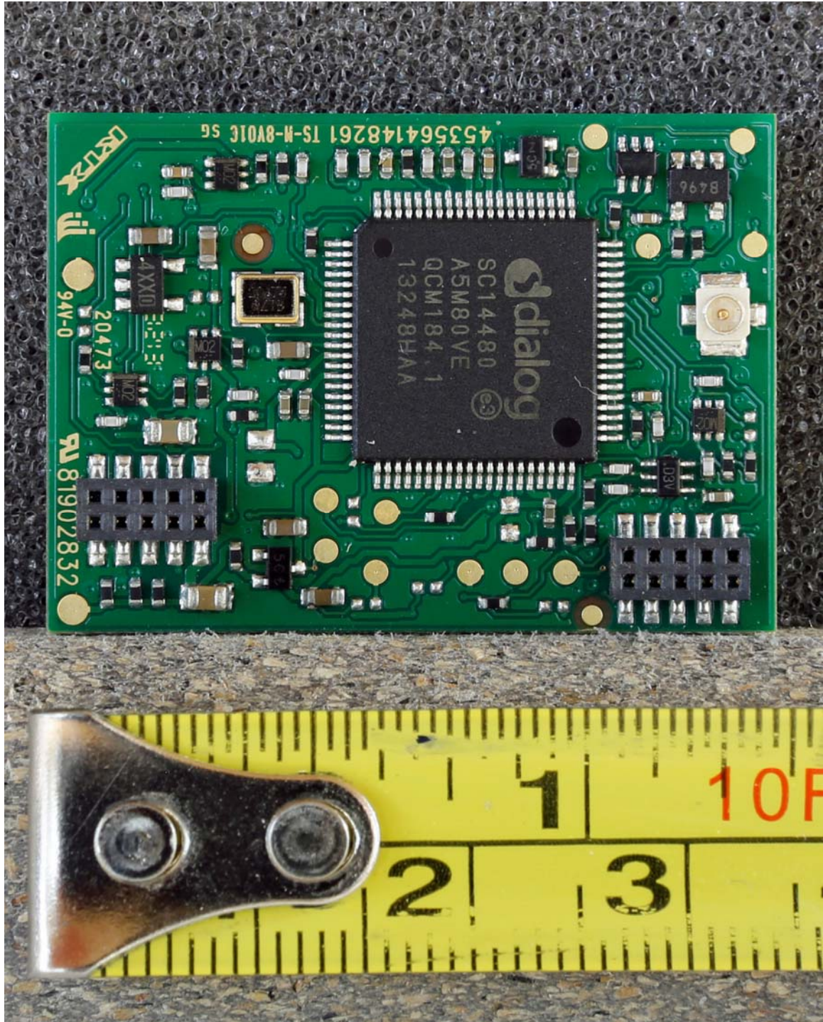
Transmitter module – Rear
