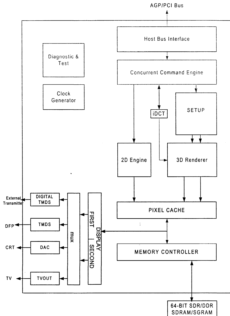
RV100-112 Functional Block Diagram
