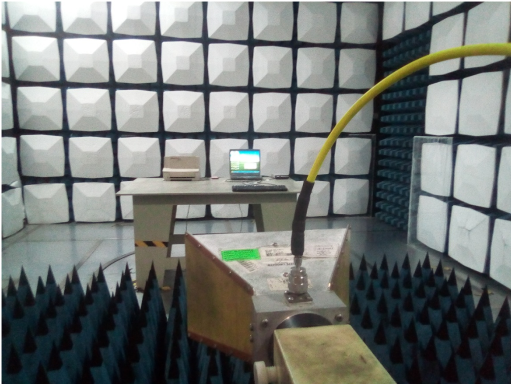
Radiated Emissions Above 1G front View
