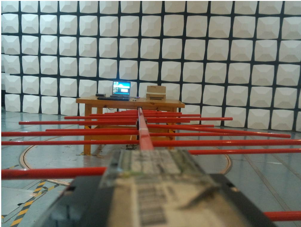
Radiated Emissions Below 1GHz Front View
