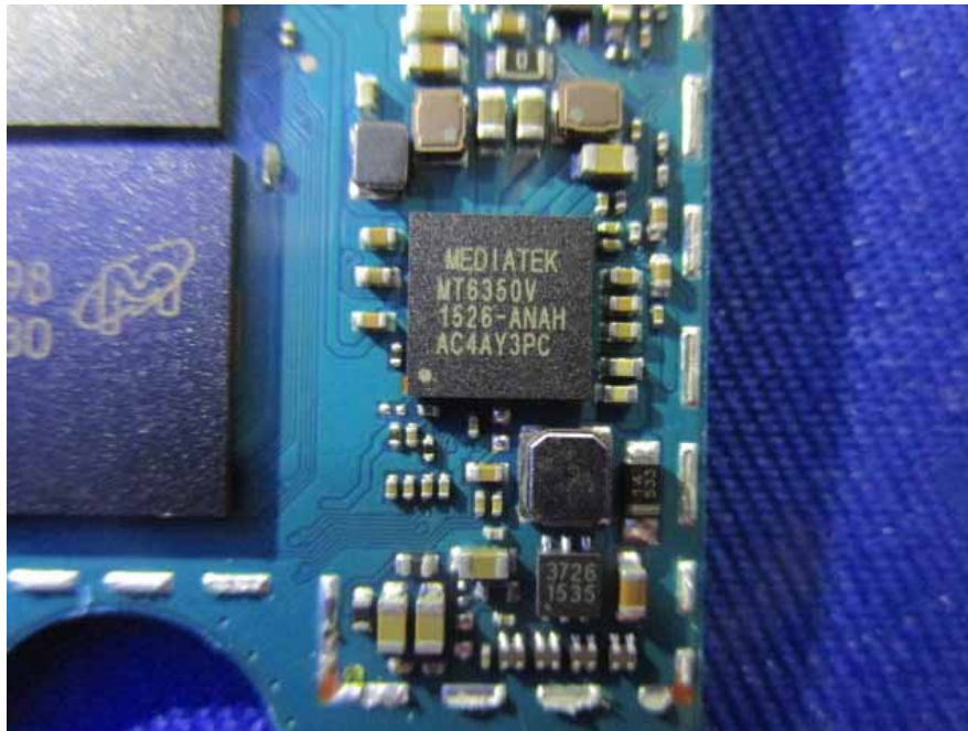
EUT –Power Management Chip View
