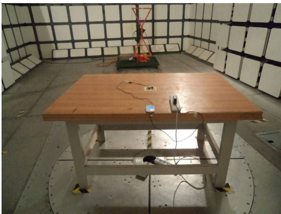
Radiated Emissions – Rear View (Charging&multimedia playing mode)
