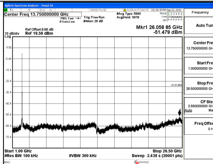
11N40SISO_Ant1_2422_0~Reference
