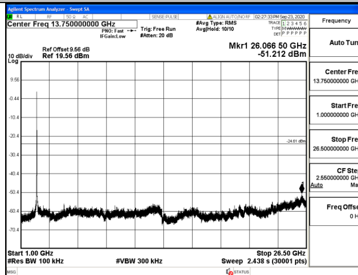
11N20SISO_Ant1_2462_0~Reference
