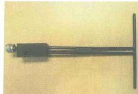
Figure 1 – MVG COMOSAR Validation Dipole
