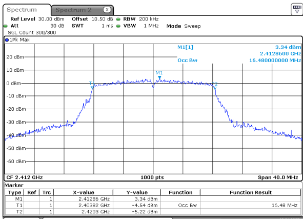
802.11g_2412MHz
