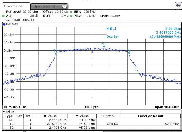
802.11g_2462MHz
