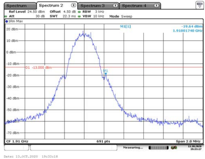
PCS 1900 Band, GSM, Right Band Edge
