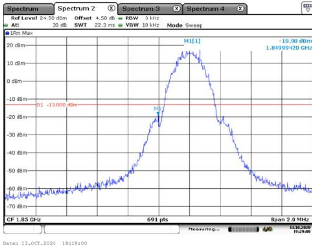
PCS 1900 Band, GSM, Left Band Edge
