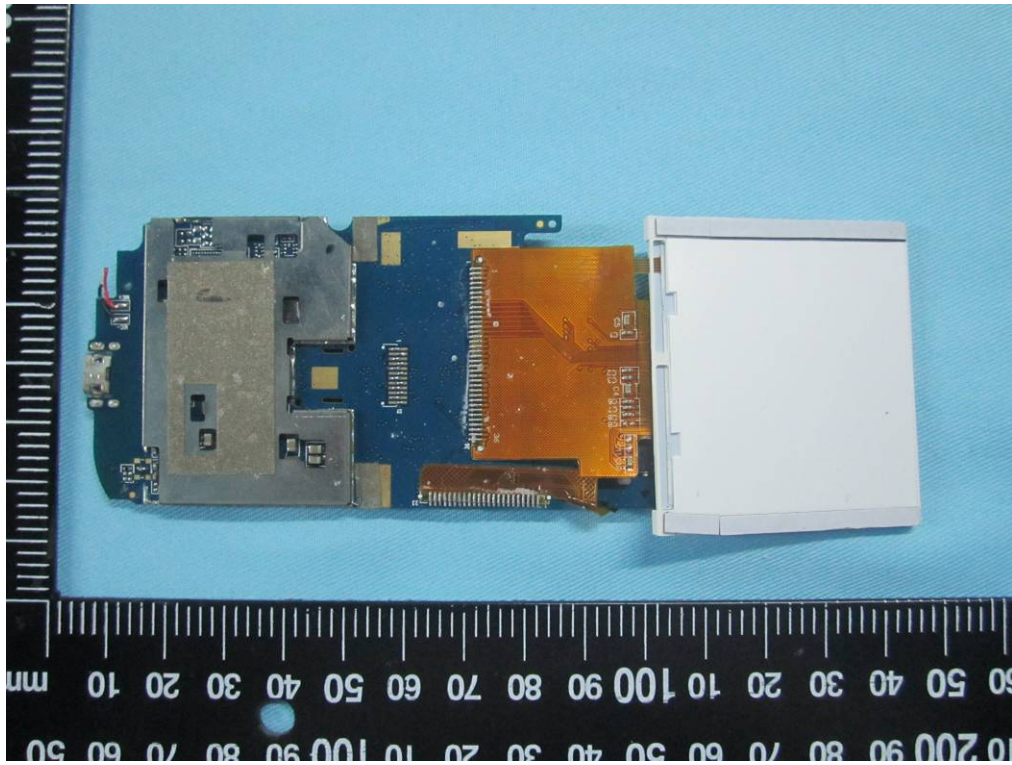
Mainboard With LCD Cover off - Front View
