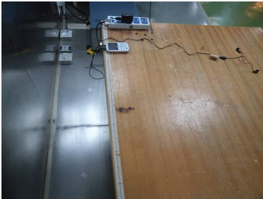
Conducted Emissions - Side View (Charging mode)
