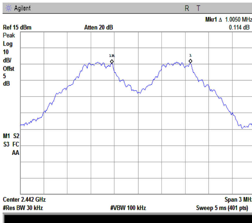
1M-Channel Separation-2441
