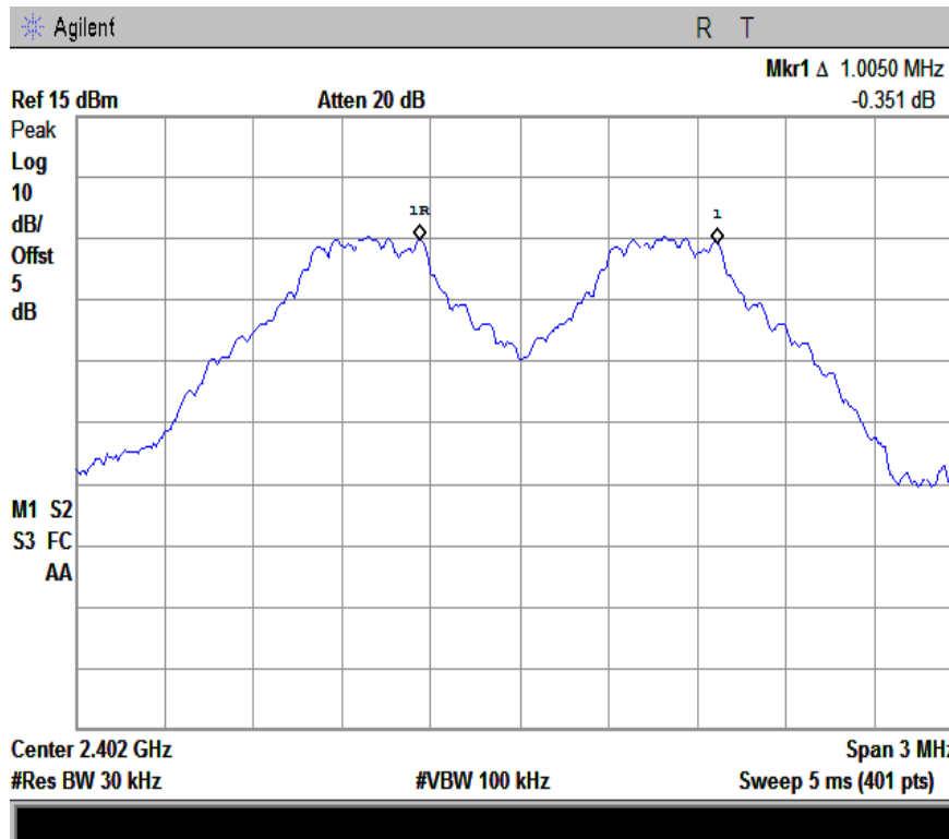
1M-Channel Separation-2402
