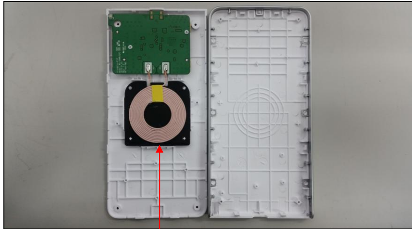
Loop Coil Antenna
