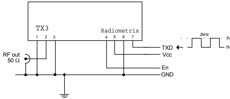
Fig.5: TX3 test circuit
