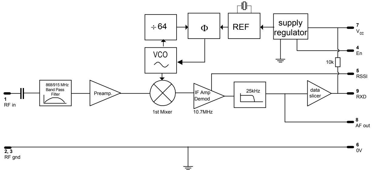
Fig.3: RX3 block diagram
