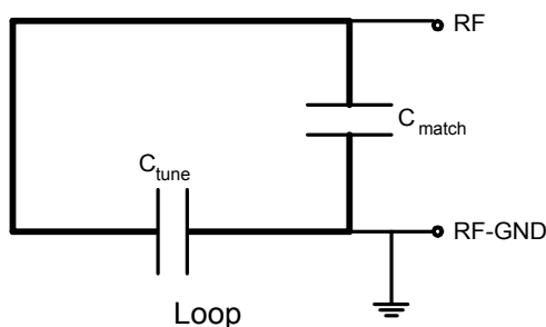
Fig.8: Integral antenna configurations
