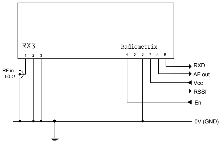
Fig.6: RX3 test circuit
