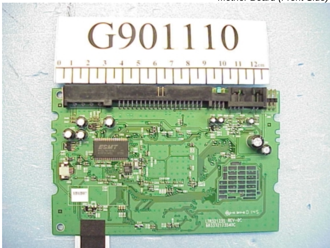
Figure 6 Mother Board (Front Side)
