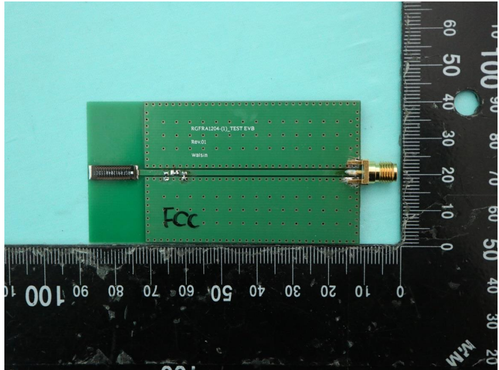
Sigfox_Chip Antenna
