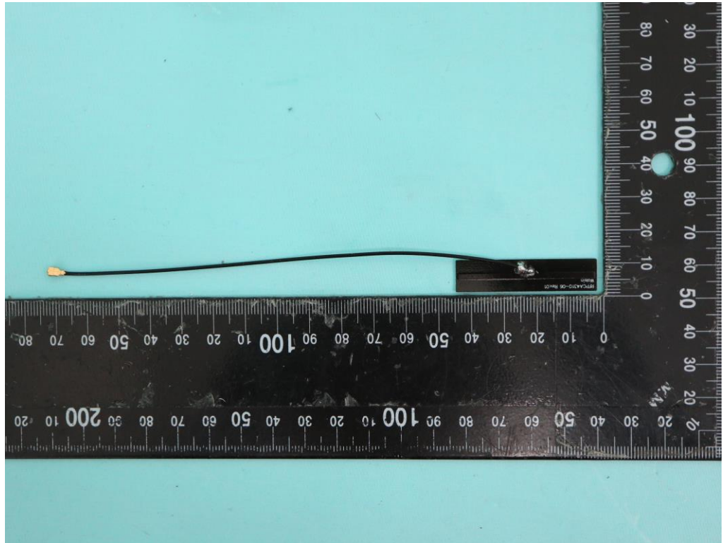
BT LE_PIFA Antenna
