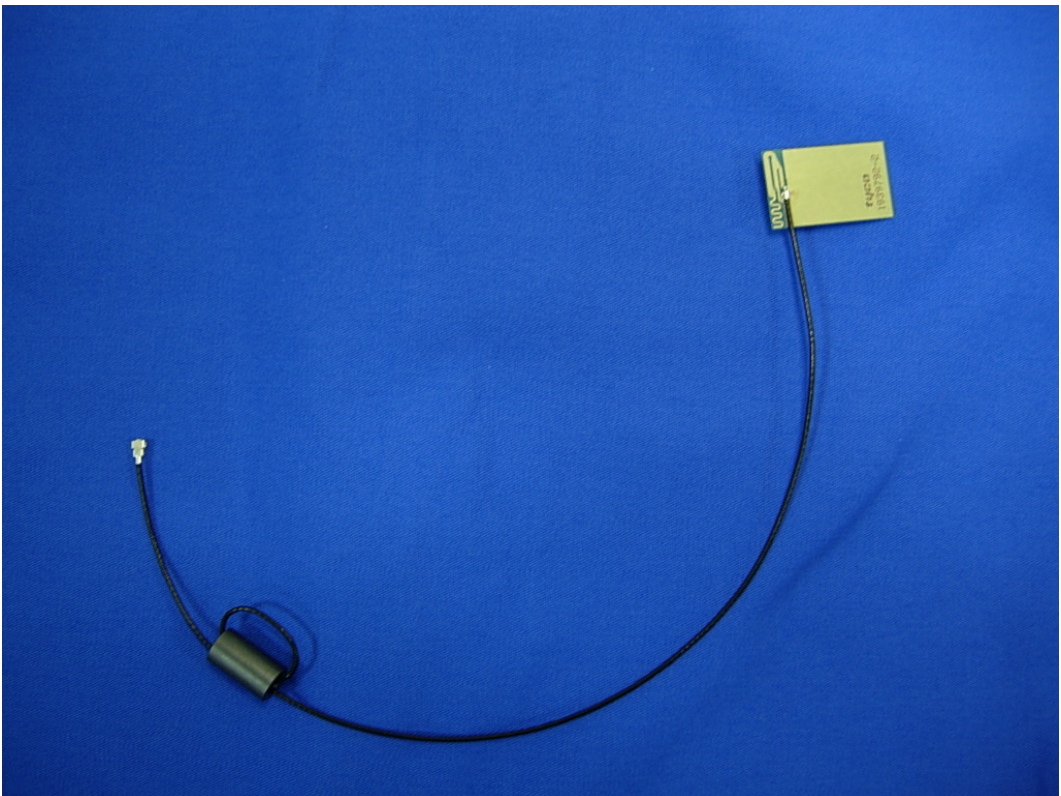
(9) EUT Photo (Antenna configure 3)
