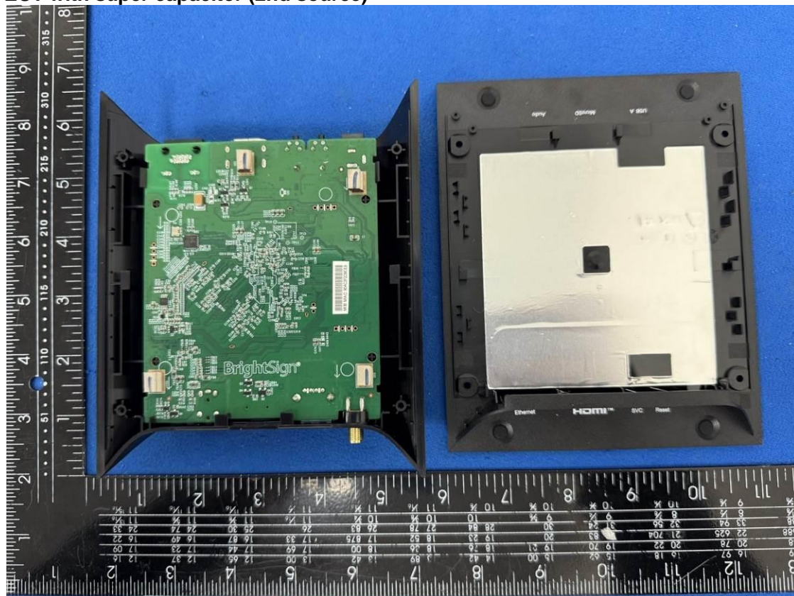
EUT with super capacitor (2nd source)
