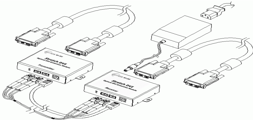
Figure 1 – Overall Optical DVI Module
