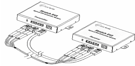
Figure 4 – Connection of 2 duplex LC fiber cables
