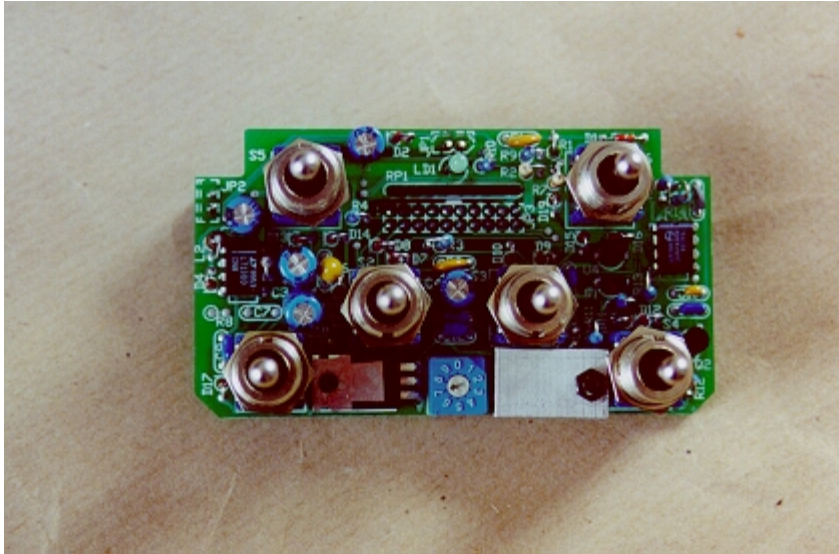
Switch board component side
