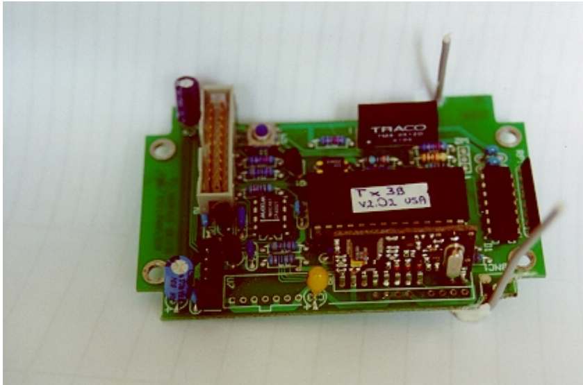
RF board Component side
