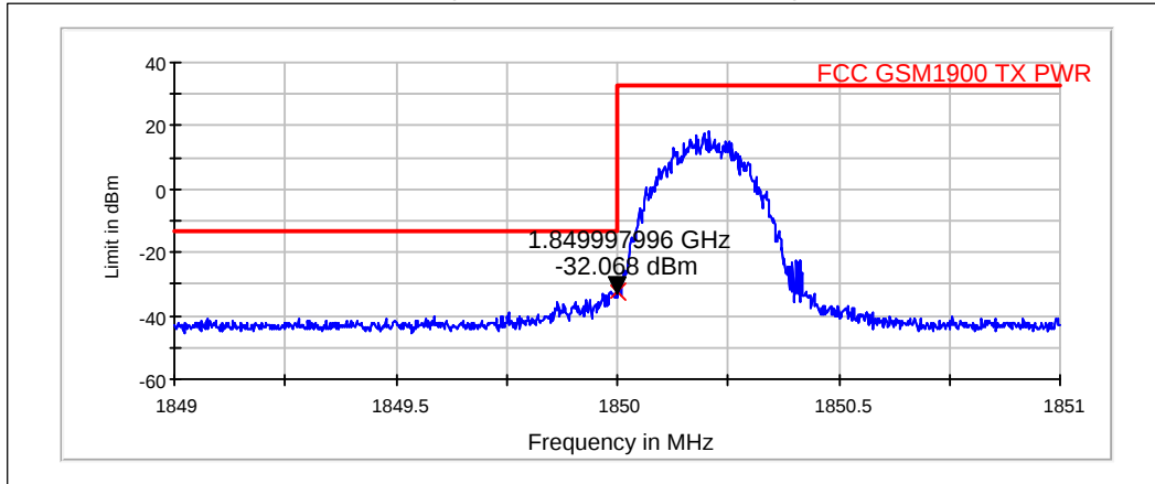
EGPRS, channel 512 / 1850.2 MHz (Peak detector, RBW: 3 kHz)
