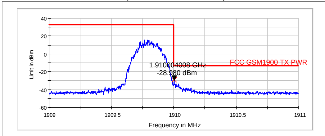
EGPRS, channel 810 / 1909.8 MHz (Peak detector, RBW: 3 kHz)
