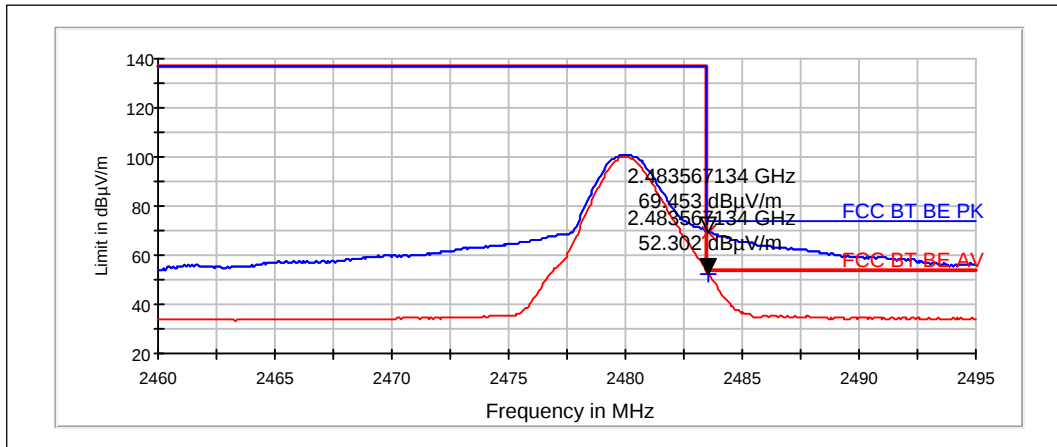
GFSK mode. Channel 78 / 2480 MHz
