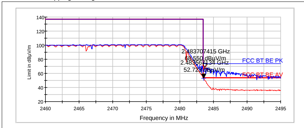
GFSK mode. Hopping on, high end
