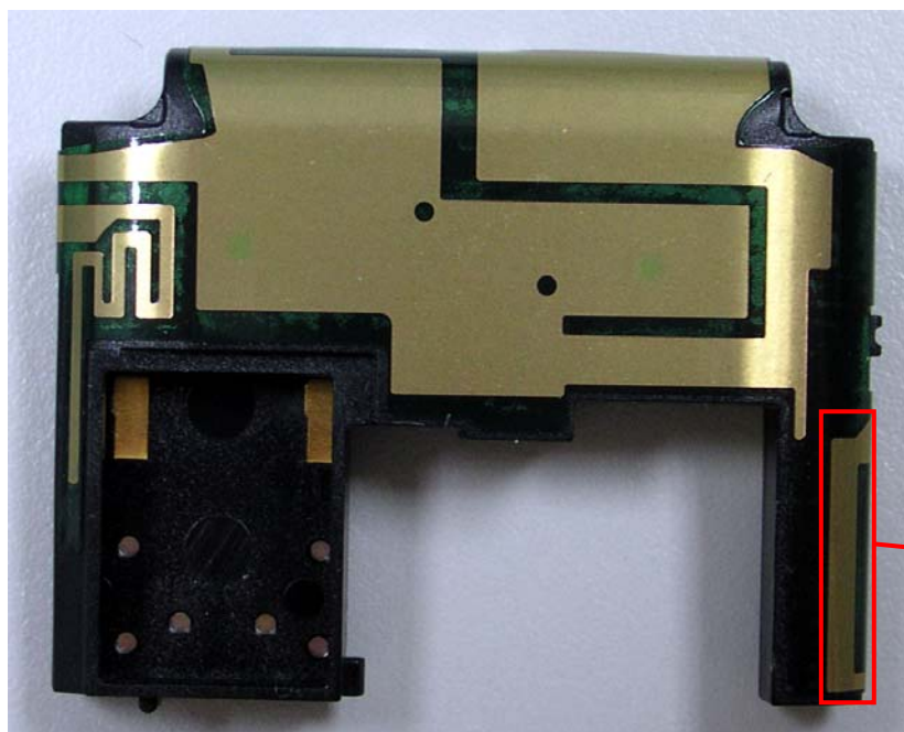
BT antenna contact
