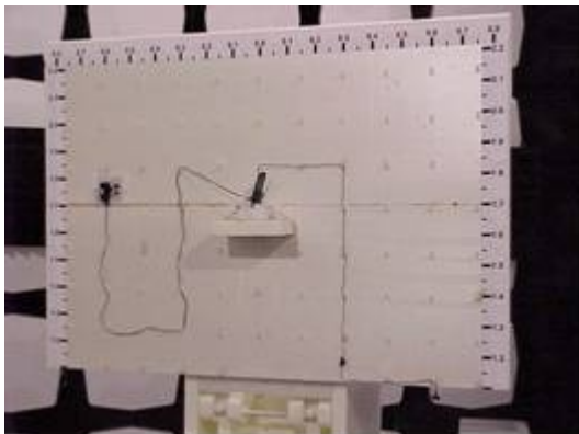
Picture 1. FCC Part 15C Radiated emissions
