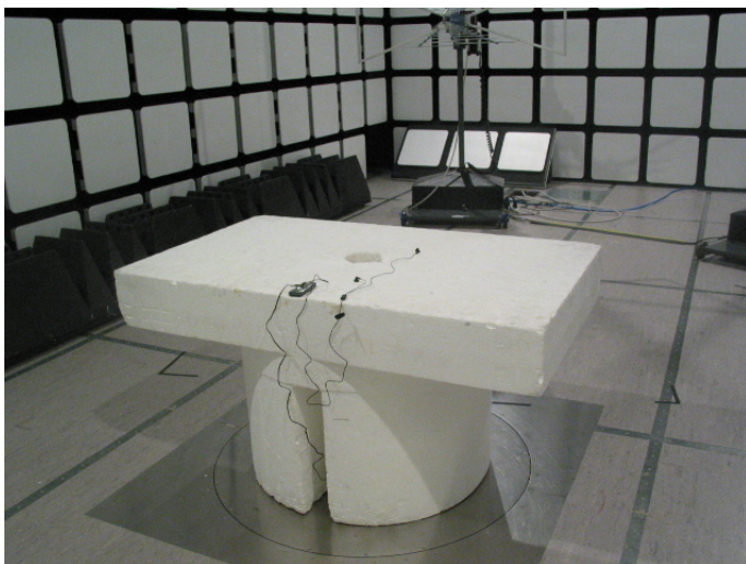
Picture 3 Radiated emission measurement Bluetooth TX / FM radio on
