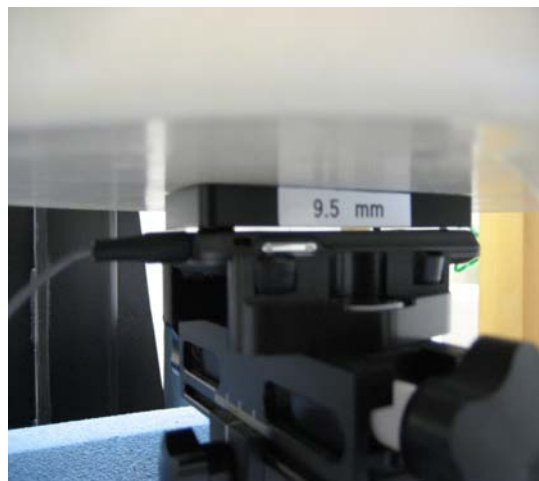
Photo of the device positioned for Body SAR measurement. The spacer was removed for the tests.
