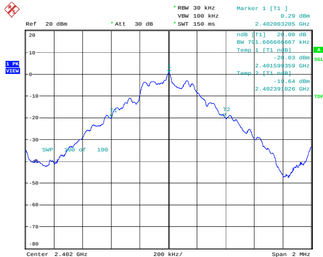
Channel 0 / 2402 MHz
