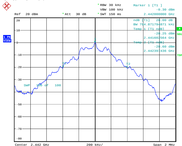
Channel 40 / 2442 MHz
