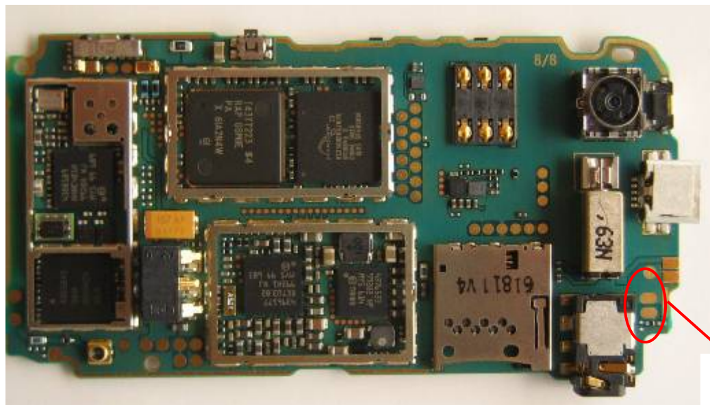
BT antenna feeding points
