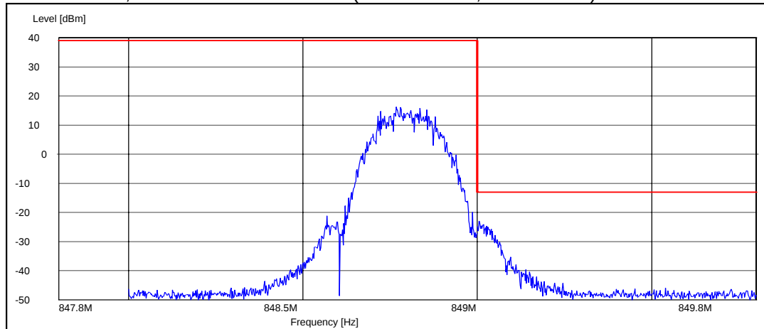
EGPRS mode, channel 251 / 848.8 MHz (Peak detector, RBW: 3 kHz)
