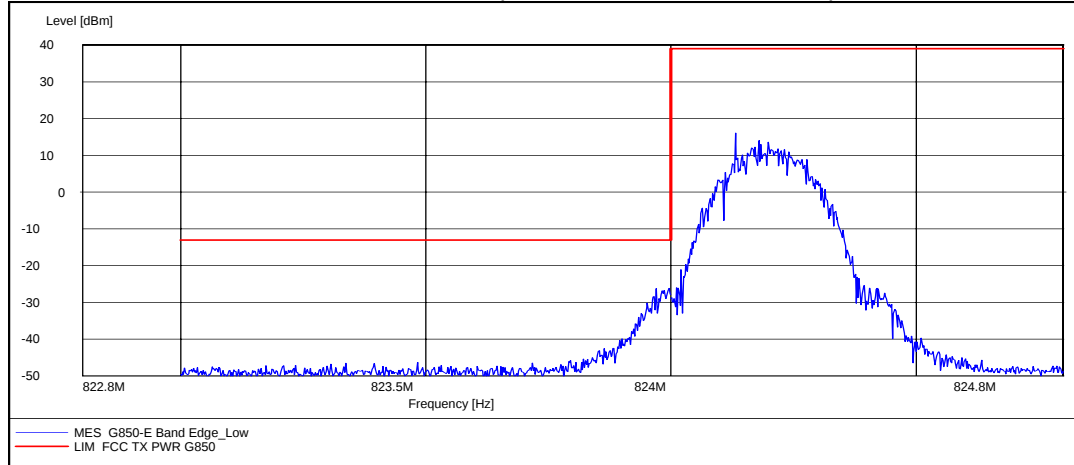
EGPRS mode, channel 128 / 824.2 MHz (Peak detector, RBW: 3 kHz)
