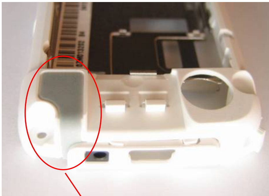
BT Antenna
