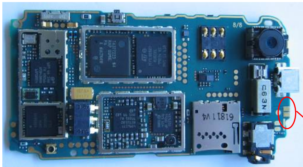
BT antenna feeding points
