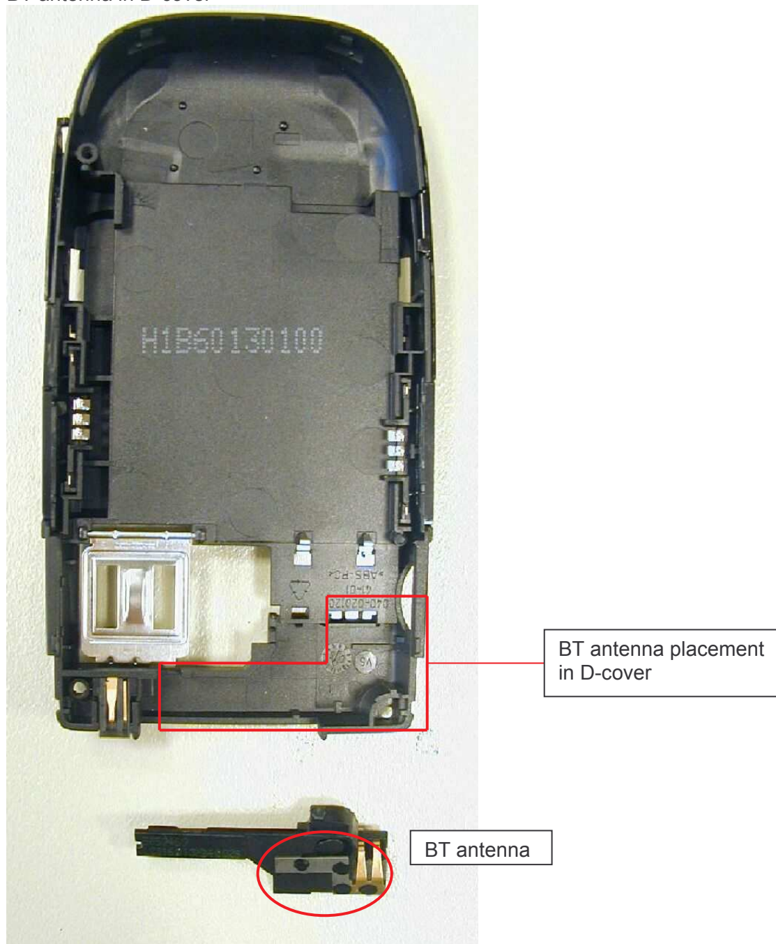
BT antenna in D-cover
