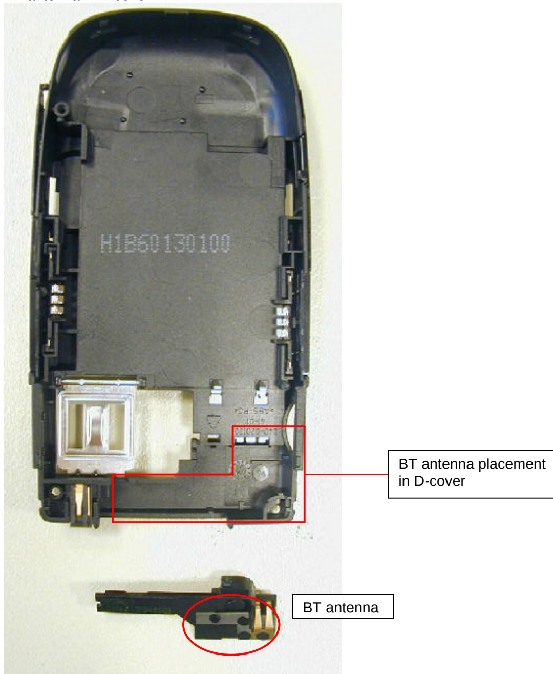
BT antenna in D-cover
