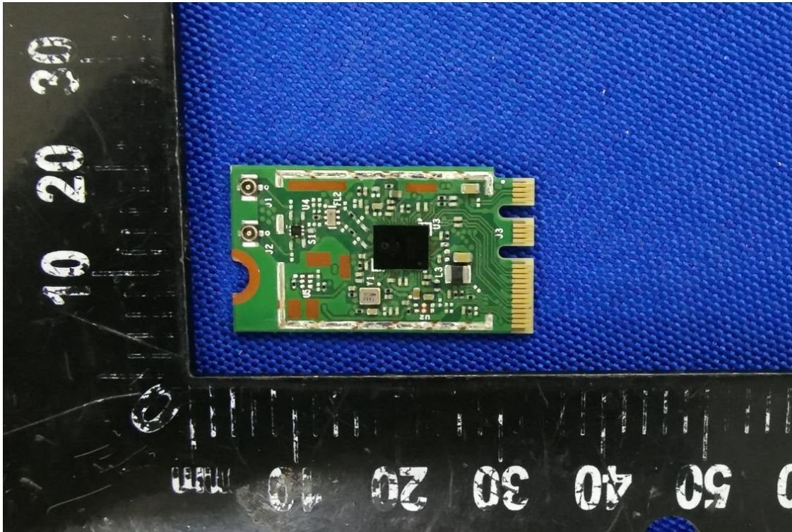
RF MODULE TOP VIEW (WITHOUT SHIELDING)
