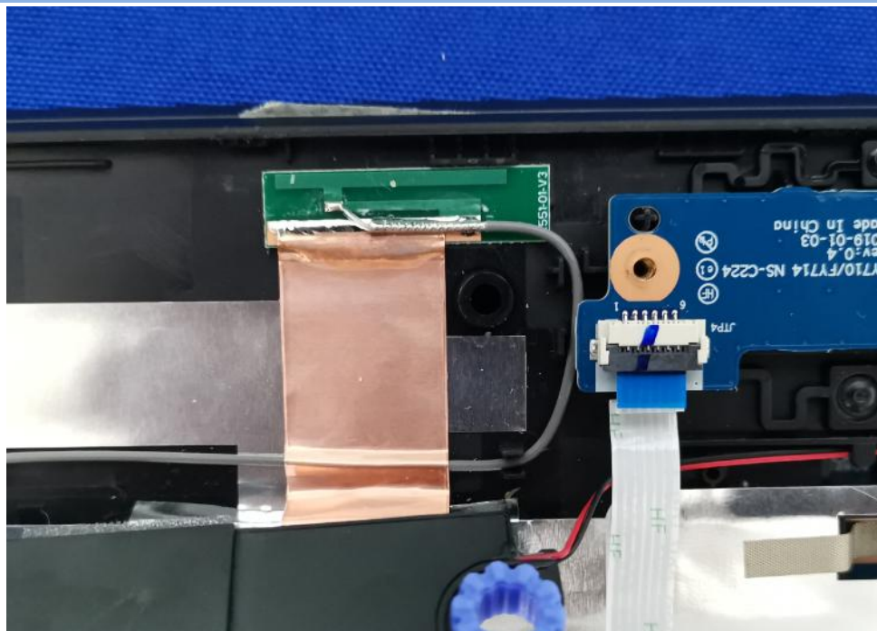
ANTENNA PHOTO (AUX ANTENNA)
