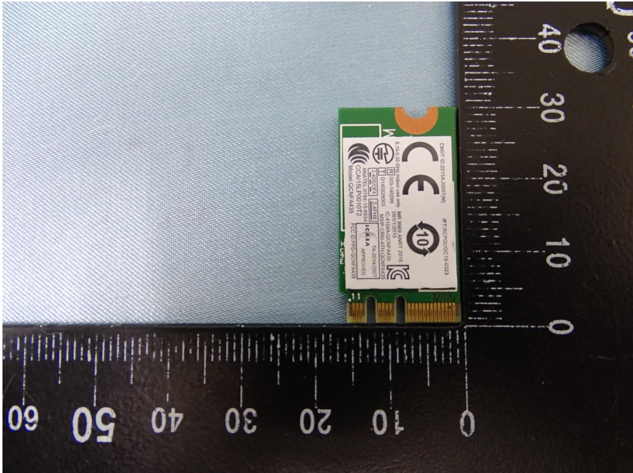
EUT: Wireless Module (Brand Name: Qualcomm / Model Name: QCNFA435)
