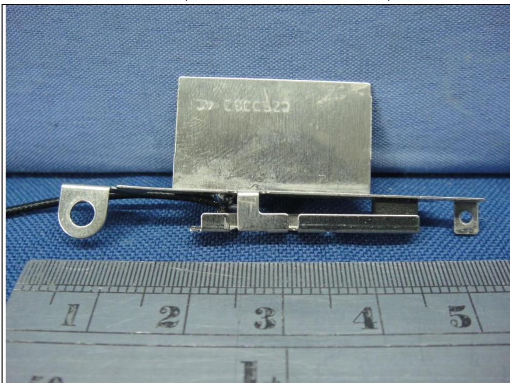
Antenna (Model : 81.EBJ15.005 <Aux>)
