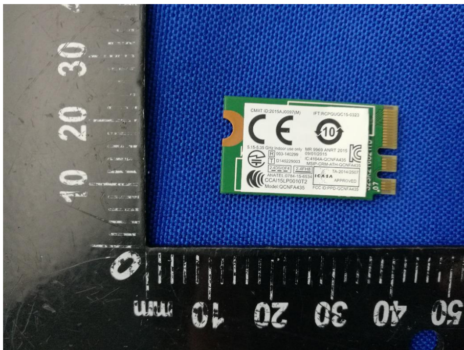
RF MODULE BACK VIEW
