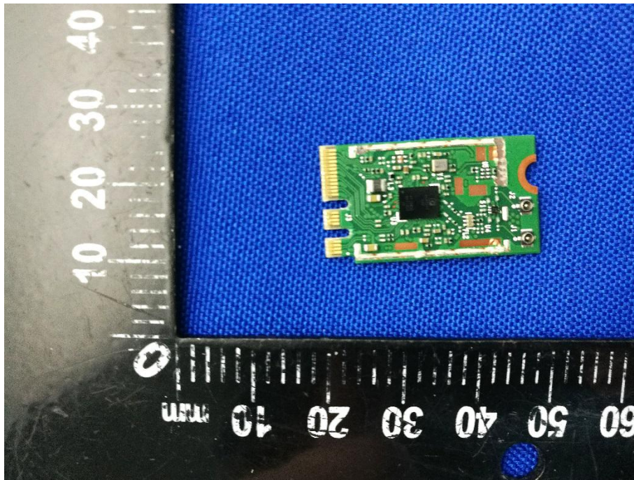
RF MODULE TOP VIEW (WITHOUT SHIELDING)
