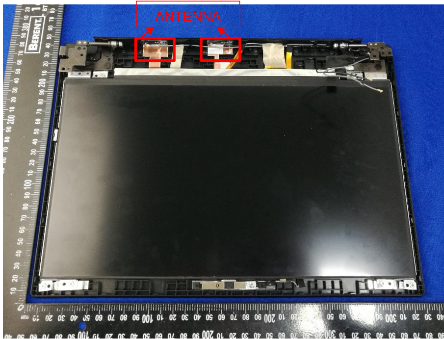
ANTENNA PHOTO 1
