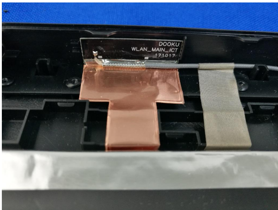
ANTENNA PHOTO 2
