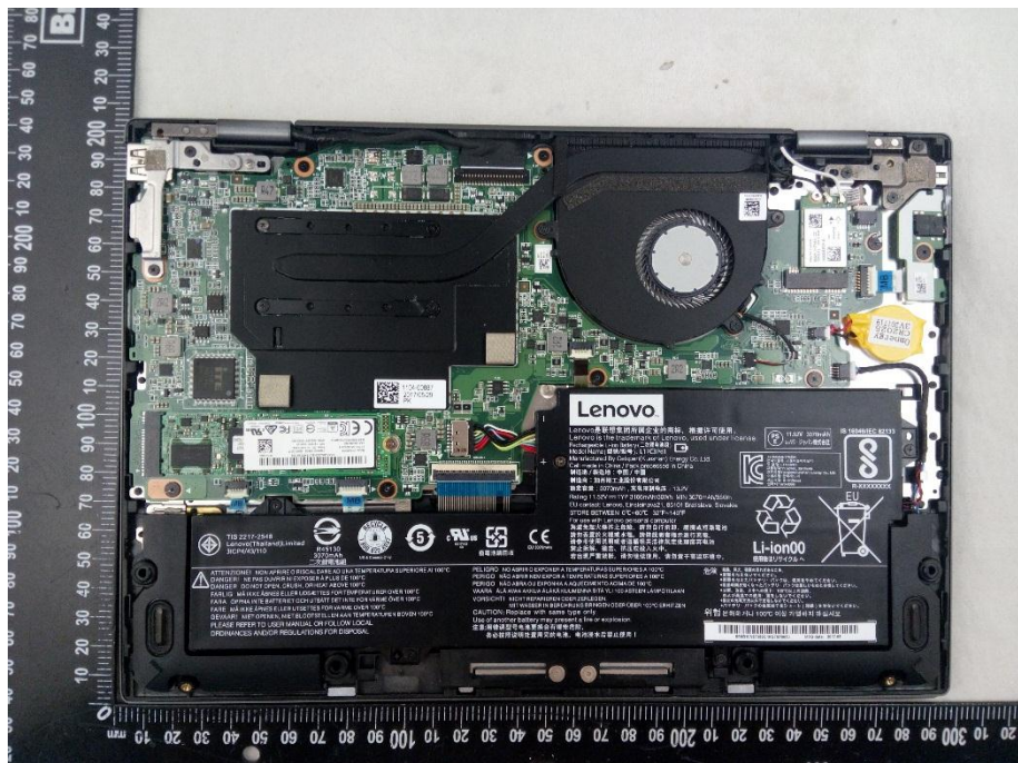
HOST UNCOVER VIEW 1
