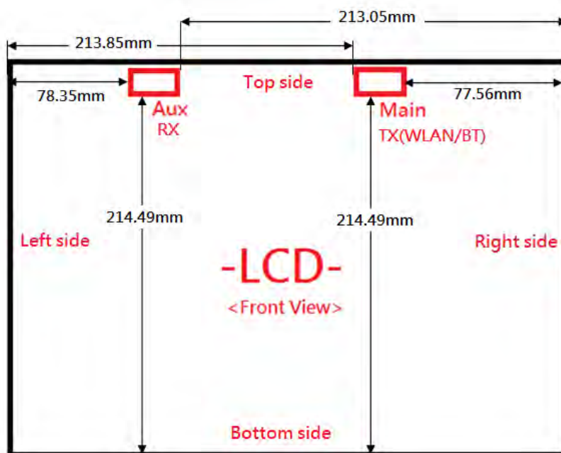
Fig.7 Antenna location of tablet mode (Front view)
