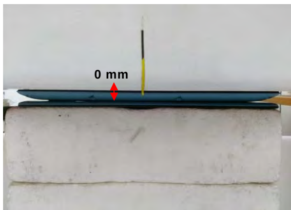
Fig.4 EUT Back side (tablet mode) to flat phantom
