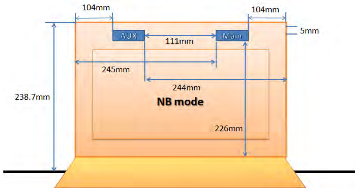
Fig.7 Antenna position of EUT
