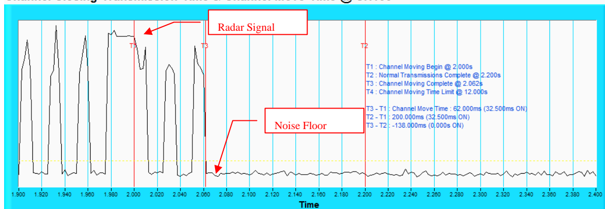
Channel Closing Transmission Time & Channel Move Time @ CH100
