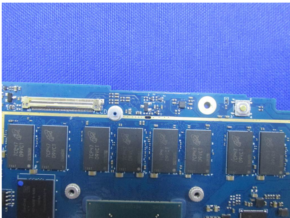
(12) EUT Photo Memory(Micron/MT41K256M16TW-107:P)
