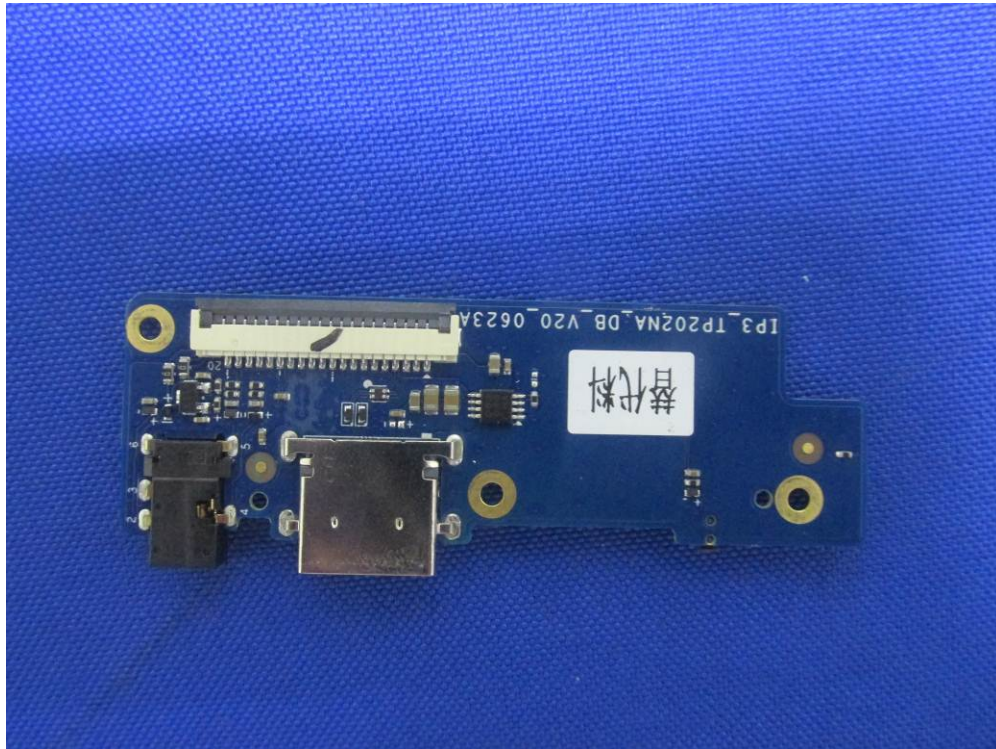
(7) EUT Photo Otherboard
