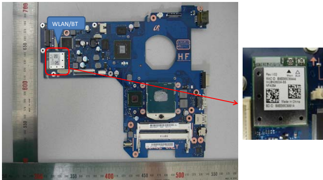
Main Board Top
