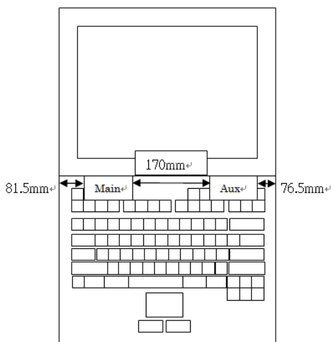
Fig.7 Antenna position of EUT (Front view)
