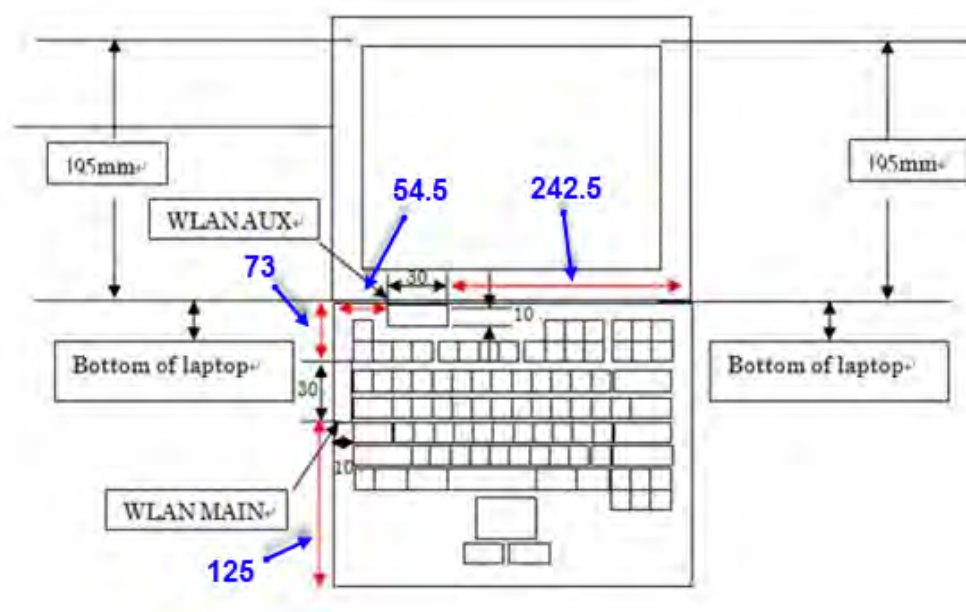
Fig.7 Antenna position of EUT (Front view)
