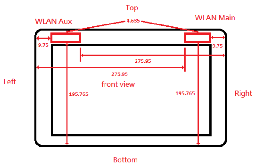
Fig.9 Antenna location of EUT (tablet mode)
