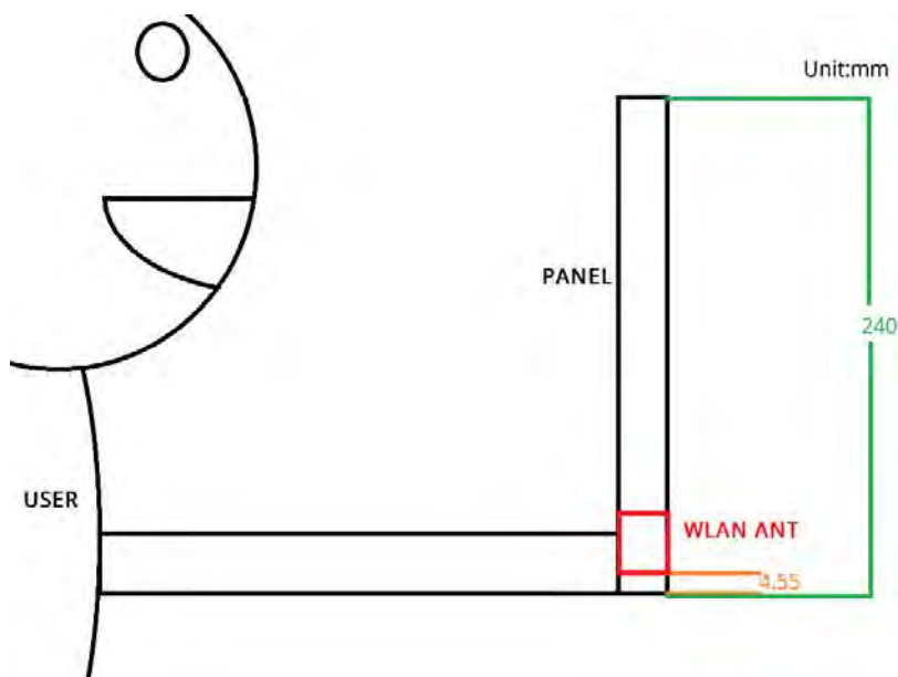
Fig.10 Antenna location of EUT
