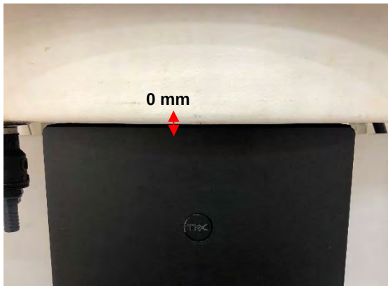
Fig.4 EUT Bottom side to flat phantom (Magnesium alloy)
