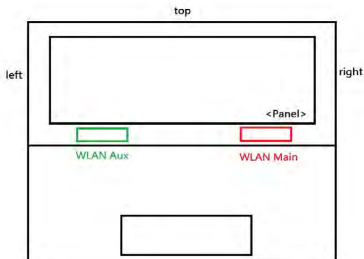
Fig.9 Antenna location of EUT (laptop mode)
