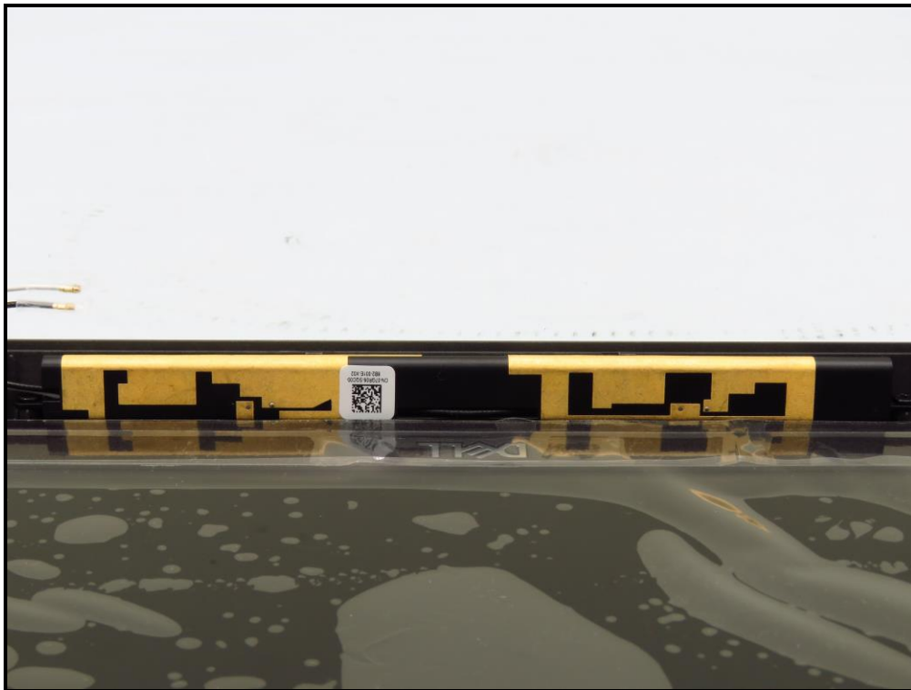
*Speed antenna (material: CF)
